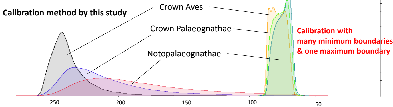
C Prior distribution of the divergence times (rooted tree)
